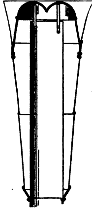
Fig. 190. Dripps Smoke Stack Applied to Locomotive John Bull in 1831
