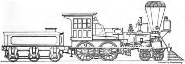
Fig. 147. One of Baldwin's First 4-4-0 for Pennsylvania Railroad
