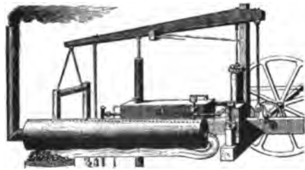
Fig. 9. Evans Columbia Engine
