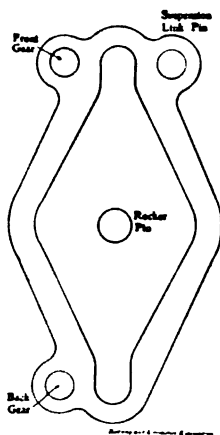
Fig. 216. Rogers Connected Double Hook
