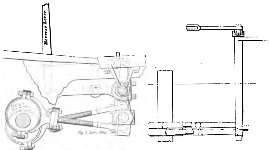
Fig. 233. Baldwin's First Link Motion in 1845
