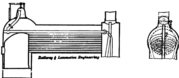
Fig. 167. Bury Boiler, 1840.
