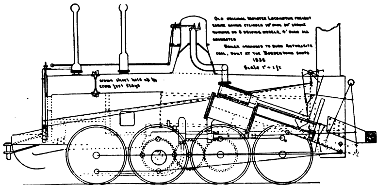
Fig. 51. Original Monster
