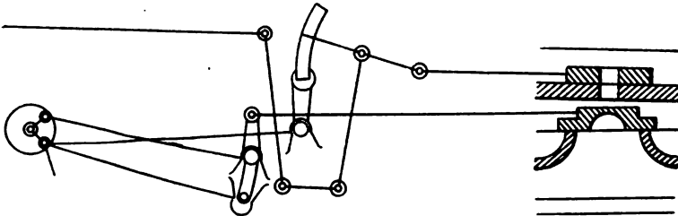
Fig. 219. Cuyahoga Cut-Off, 1850
