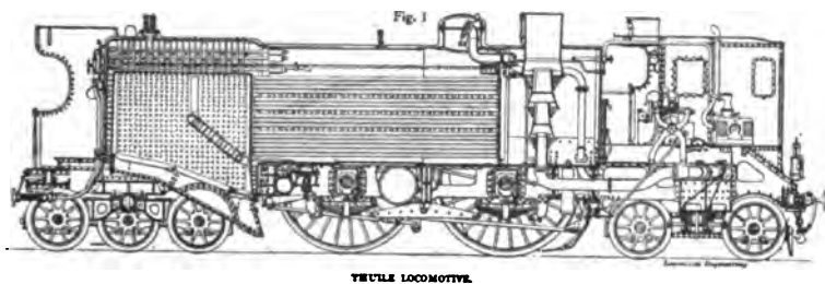
Fig. 259. Thuile Locomotive
