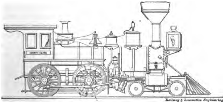
Fig. 105. Famous Morrill Engine, Built by Vermont Central Railroad About 1863 From drawing loaned by R. E. Russell, Burlington, Vt.
