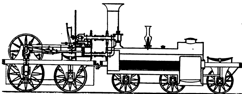
Fig. 247. Harrison's "Thunderer"
