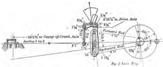
Fig. 234. Allan's Straight Link
