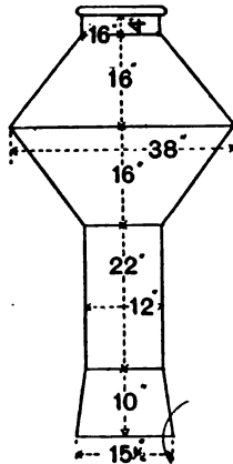
First Diamond Stack Ever Made
