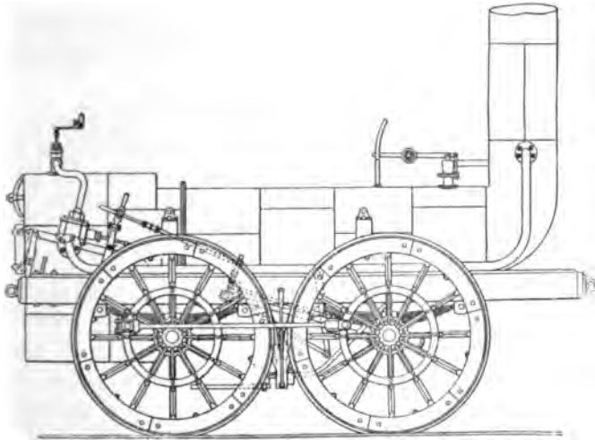
Fig 32. The "West Point"
