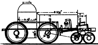
Fig. 118. Rogers' Sullivan First Engine for Erie
