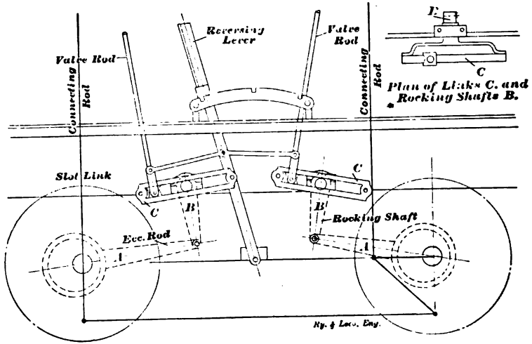
Fig. 267. Modernized Valve Motion
