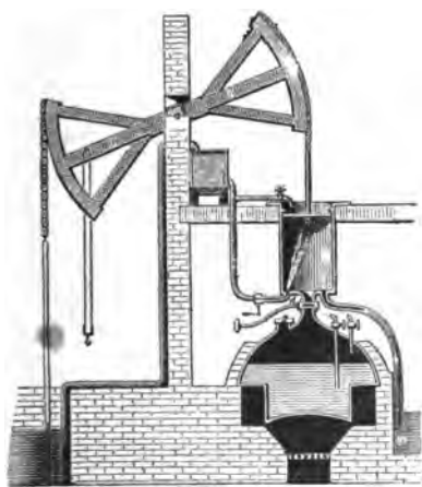
Fig. 4. Newcomen's Engine
