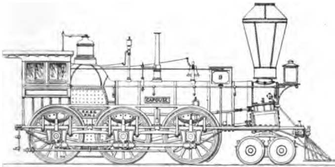
Fig. 129. Lackawanna's First Freight Engine, 1851
