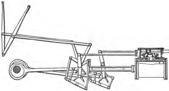
Fig. 221. Rogers' Valve Motion
