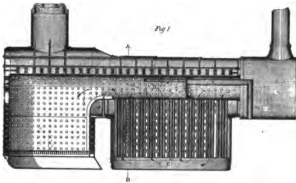
Fig. 185. Boardman's Boiler
