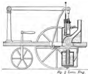
Fig. 8. Murdoch's Model
