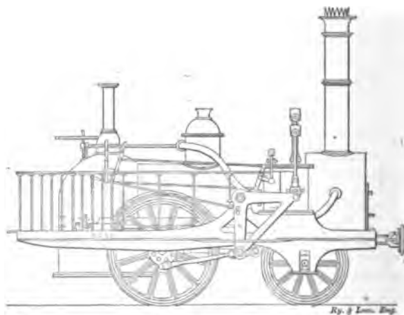
Fig. 242. Roberts' Experiment, 1833
