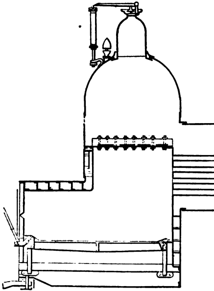
Fig 121. Winans' Firebox
