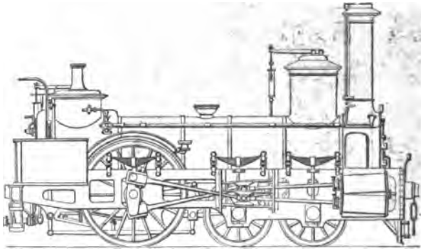
Fig. 250. "Duplex," Austria, 1861
