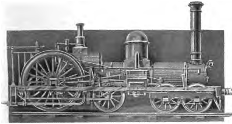
Fig. 58. Lightning, Built by Edward S. Norris at Schenectady Locomotive Works, 1849
