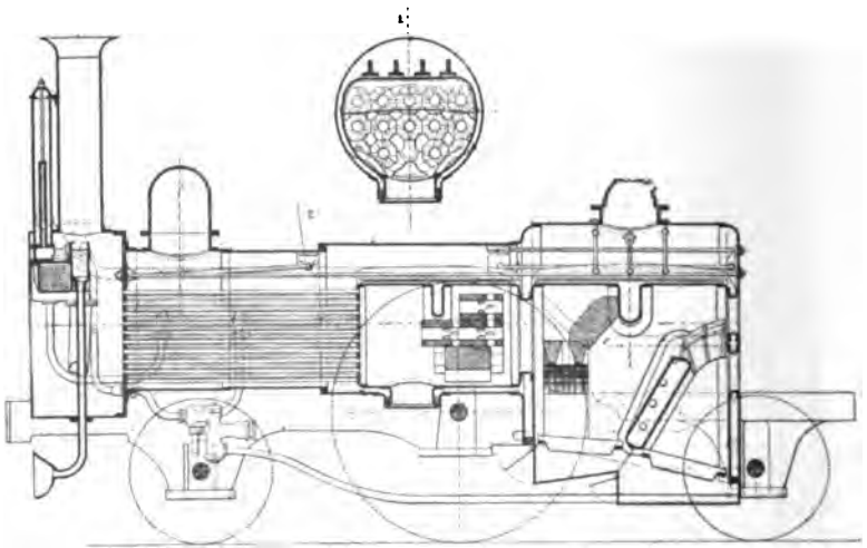
Fig. 170. Beattie's Smoke-Preventing Boiler
