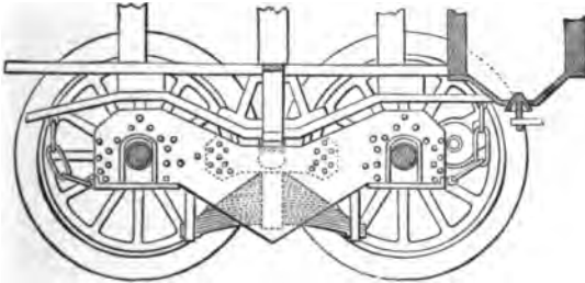
Fig. 70. Baldwin's Flexible Truck
