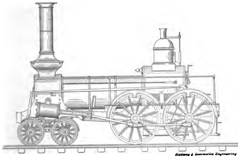
Fig. 77. Eight-Wheeler Built by Eastwick & Harrison
