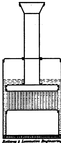
Fig. 40. Improvement on the Cheese Boiler
