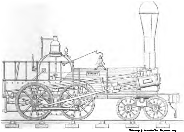
Fig. 75. Mercury
