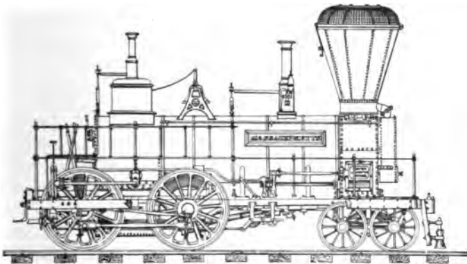
"Massachusetts," Built by Hinkley & Drury, About 1850, for Philadelphia & Reading. Cylinders, 15x 20 Inches; Drivers, 54 Inches Diameter
