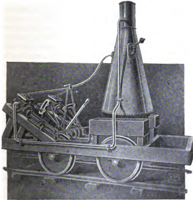
Fig. 63. James' Engine, 1832
