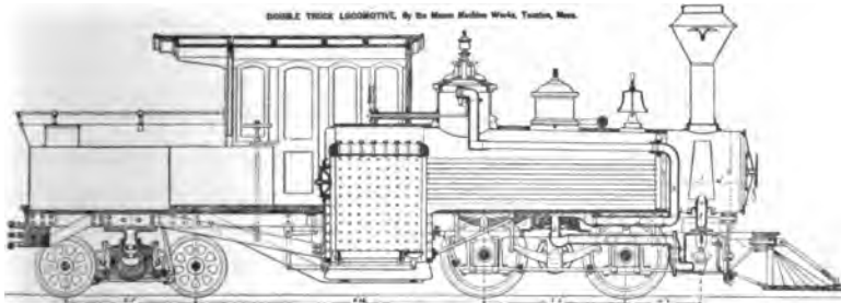
Fig. 90. Mason's Double Truck Locomotive
