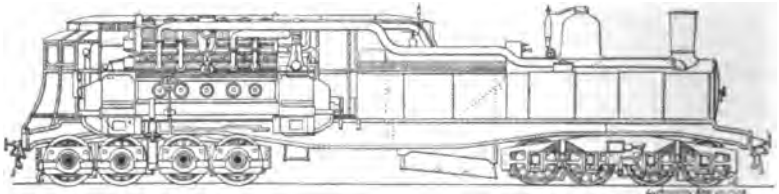
Fig. 258. Heilmann Electric Locomotive
