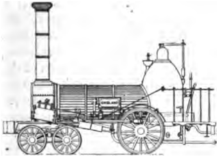
Fig. 65 Norris' England
