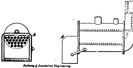
Fig. 164. Stephenson's "Rocket," 1829.
