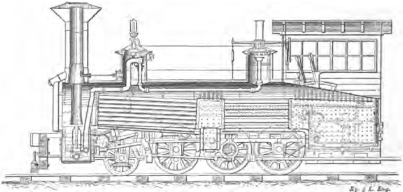
Fig. 123. Millholland's 6-Wheel Connected Engine, with His Patented Boiler (Pawnee Class)
