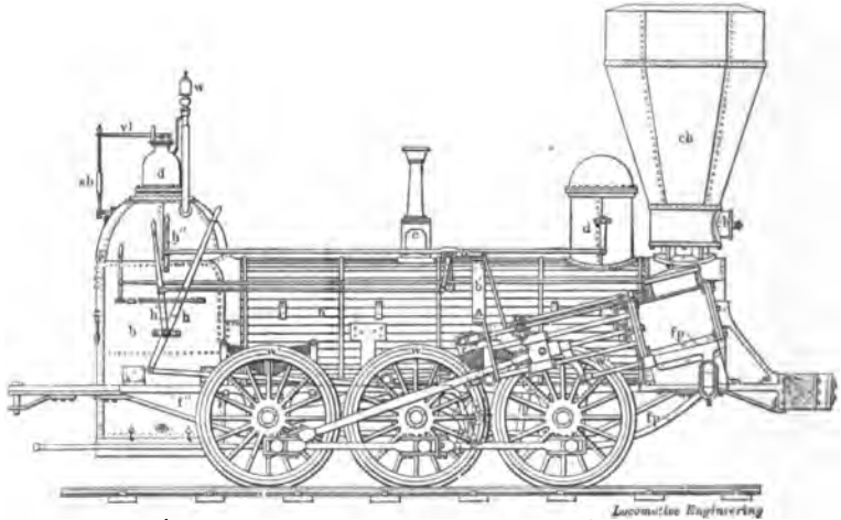
Fig. 122. Millholland's Philadelphia
