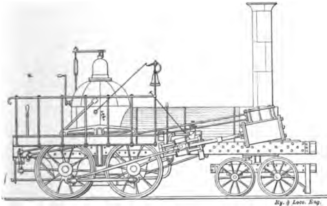
Fig. 73. Garrett & Eastwick's Locomotive Hercules
